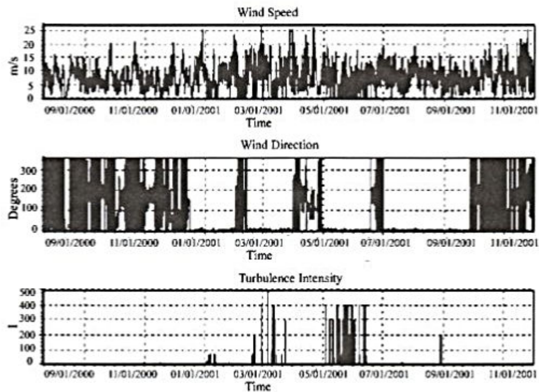
Fig. 6. Wind speed, wind direction and turbulence intensity variations at 30 m height.
