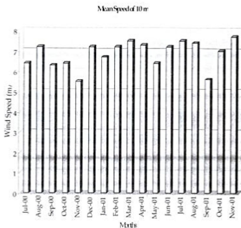
Fig. 3. Variation of monthly mean speeds at 10 m height.
