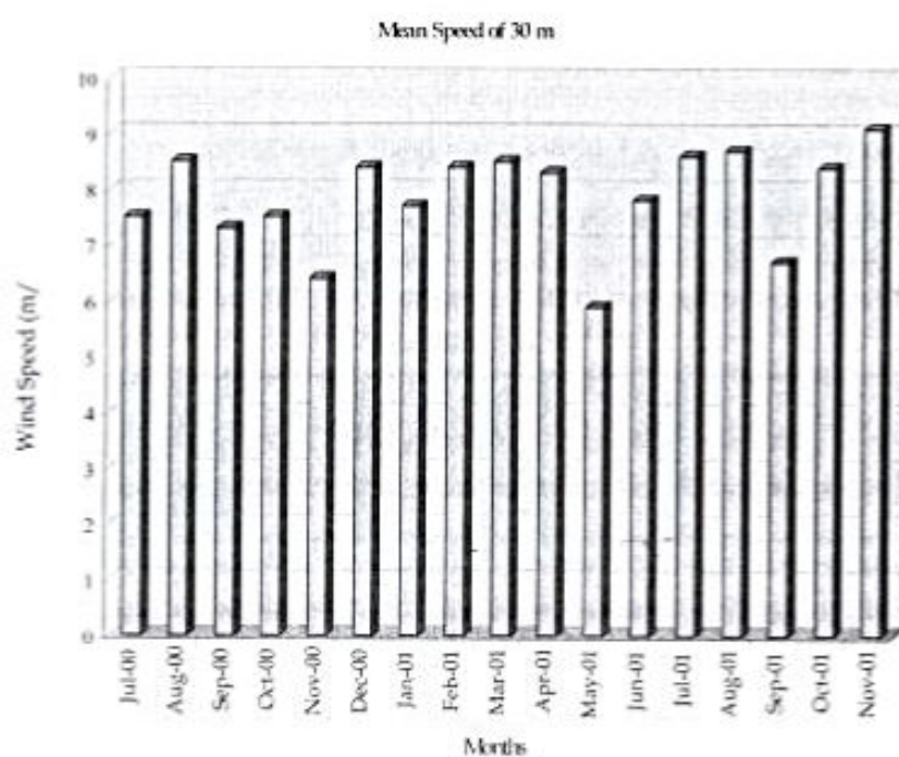
Fig. 4. Variation of monthly mean speeds at 30 m height.
