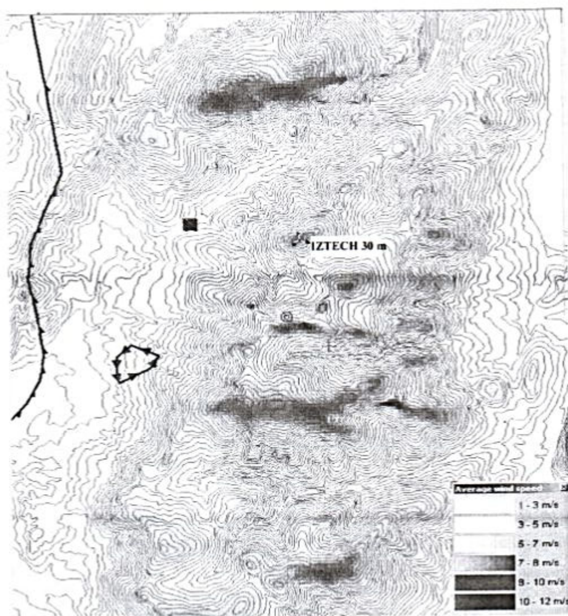
Fig. 13. Average mean speed map of the area.
