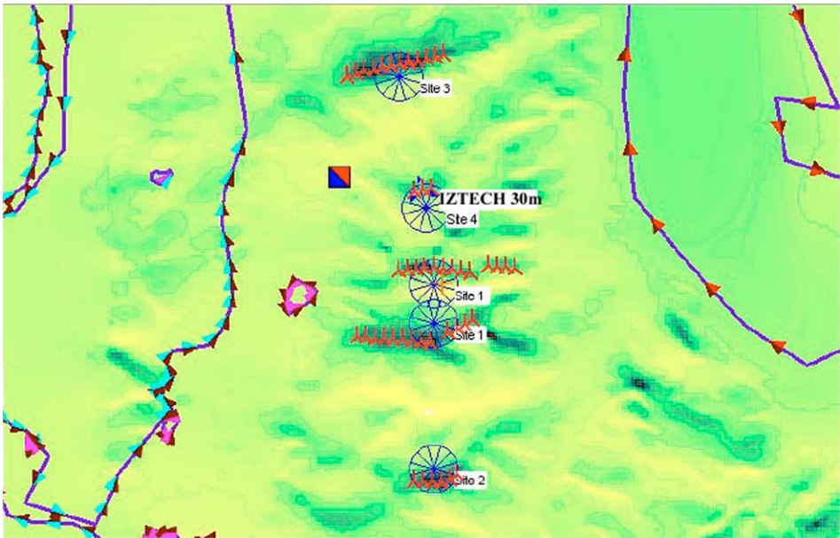
Fig. 4. Micrositting of 600 kW turbines on the campus area.
