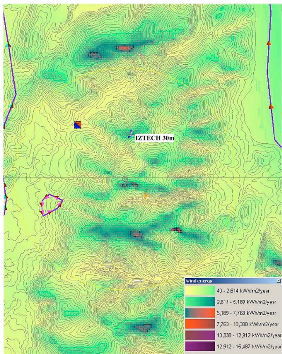
Fig. 3. Wind energy map of campus area in kWh/m²/year.
