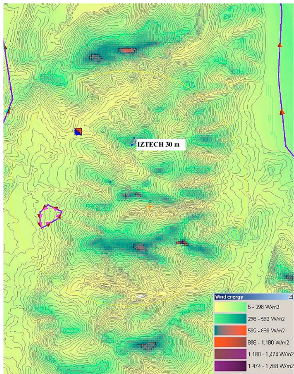
Fig. 2. Wind power map of campus area in \text{W/m}^2 .
