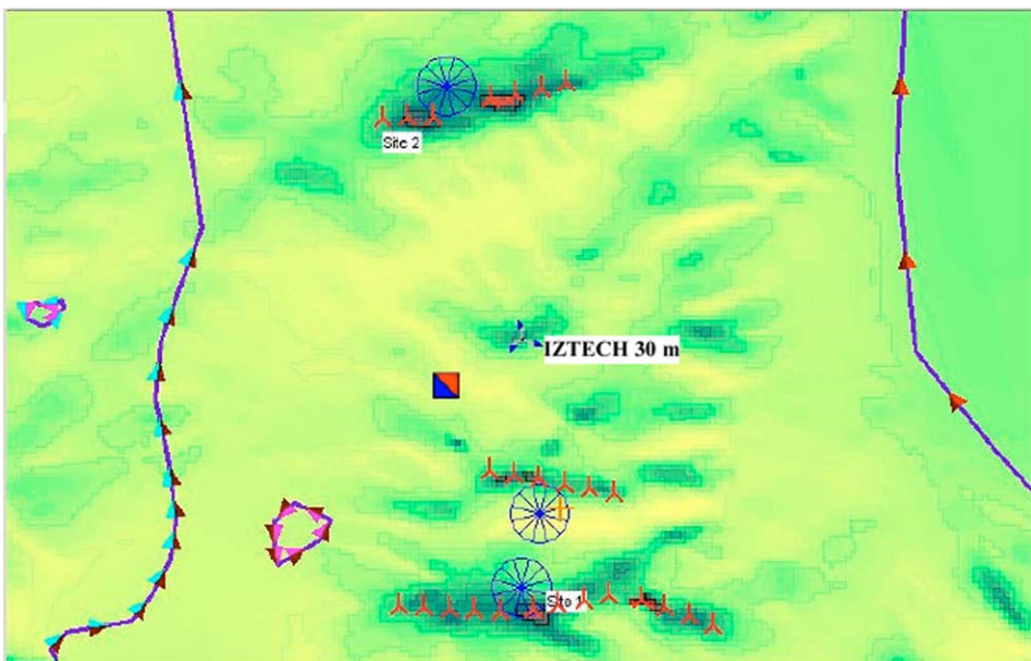
Fig. 5. Micrositting of 1500 kW turbines on the campus area.
